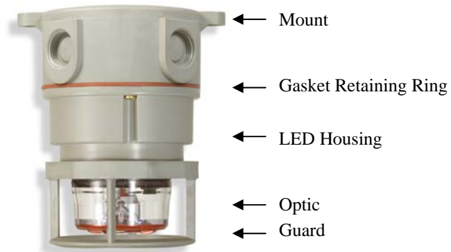
TYPICAL LED ASSEMBLY
