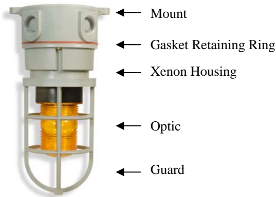
(TYPICAL XENON STROBE ASSEMBLY)
